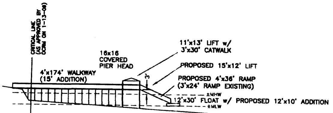
SIDE VIEW NOT TO SCALE
