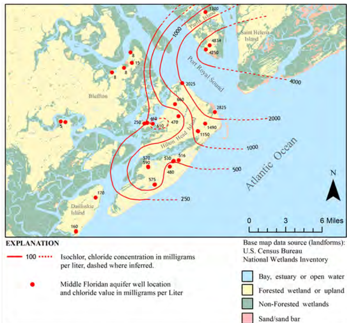
Figure 74. Chloride concentrations in pumped water samples from the middle Floridan aquifer, southern Beaufort County, S.C., 1962–2015 (data from Counts and Donsky, 1963; Back, Hanshaw, and Rubin, 1970; Gawne and Park, 1999; Groundwater Management & Associates, 2010 and 2014; and Hilton Head Island Public Service District, 2013).
