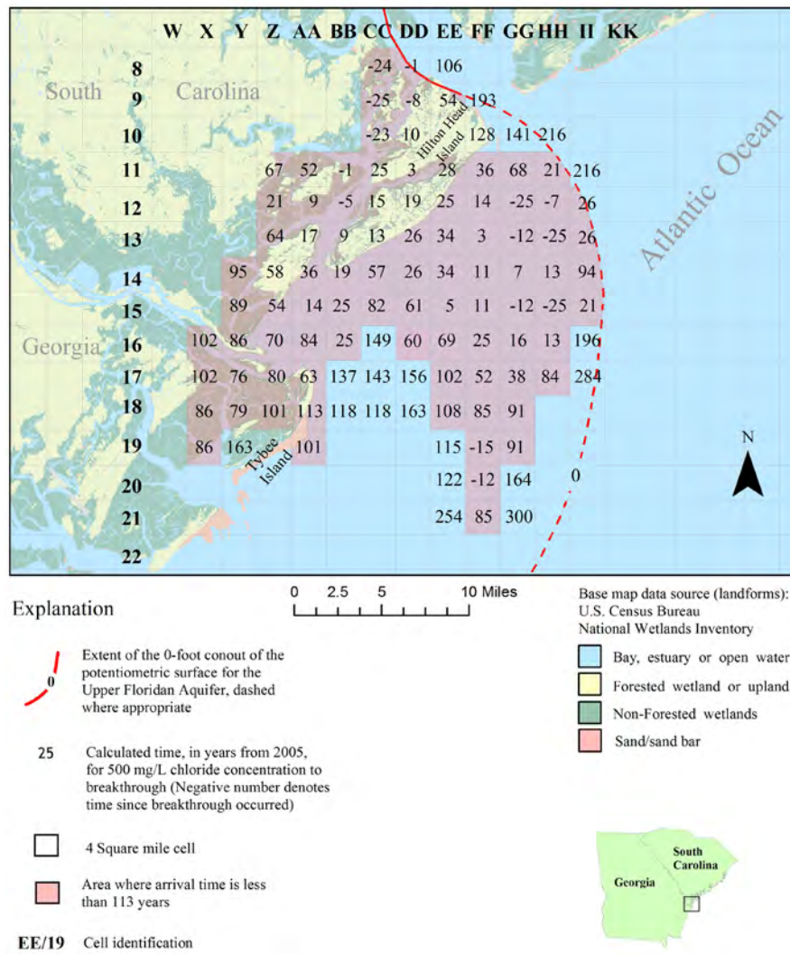
Figure 33. Estimated arrival times of a 500-mg/L chloride concentration at the top of the Upper Floridan aquifer relative to the year 2005, Savannah, Ga. – Hilton Head Island, S.C., area (Ransom and others, 2006).
