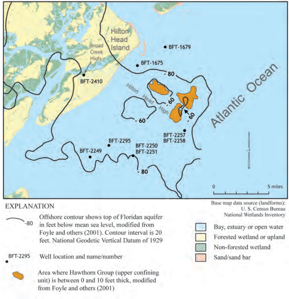
Figure 63. Locations of temporary offshore test wells near Hilton Head Island, S.C., surface contours on top of the Upper Floridan aquifer, and offshore areas where the Upper Floridan aquifer is overlain by less than 10 ft of the upper confining unit (after Foyle and others, 2001).
