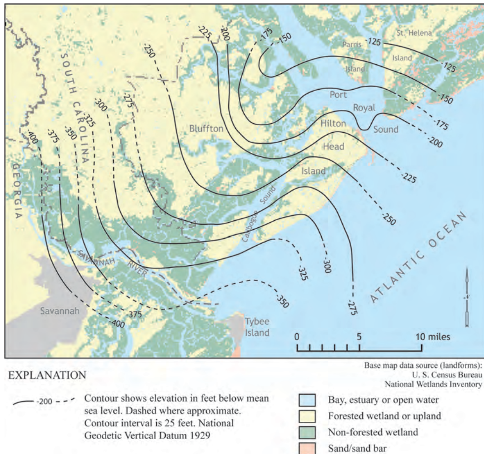
Figure 7. Structure contours showing top of lower unit of the late Eocene Ocala Limestone near Savannah, Ga., and Hilton Head Island, S.C.
