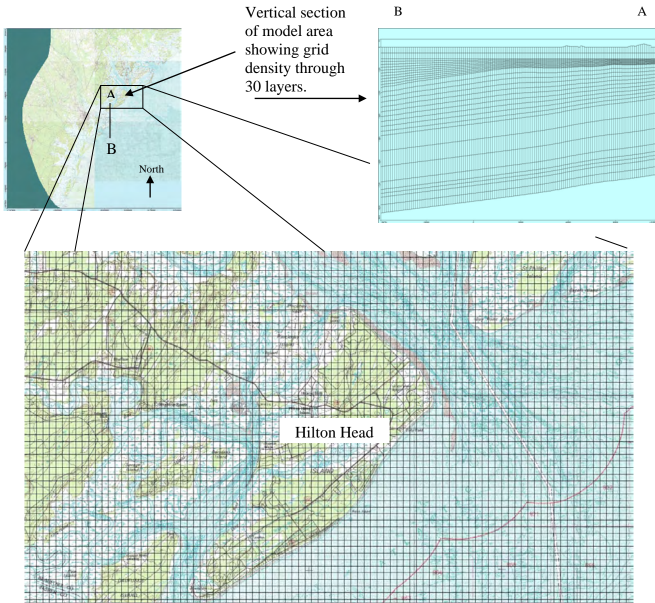
Figure J2. Map and section showing grid density for x, y, and z planes with \frac{1}{4} mi 2 cells, in part, for the model area in the vicinity of Hilton Head Island, S.C.
