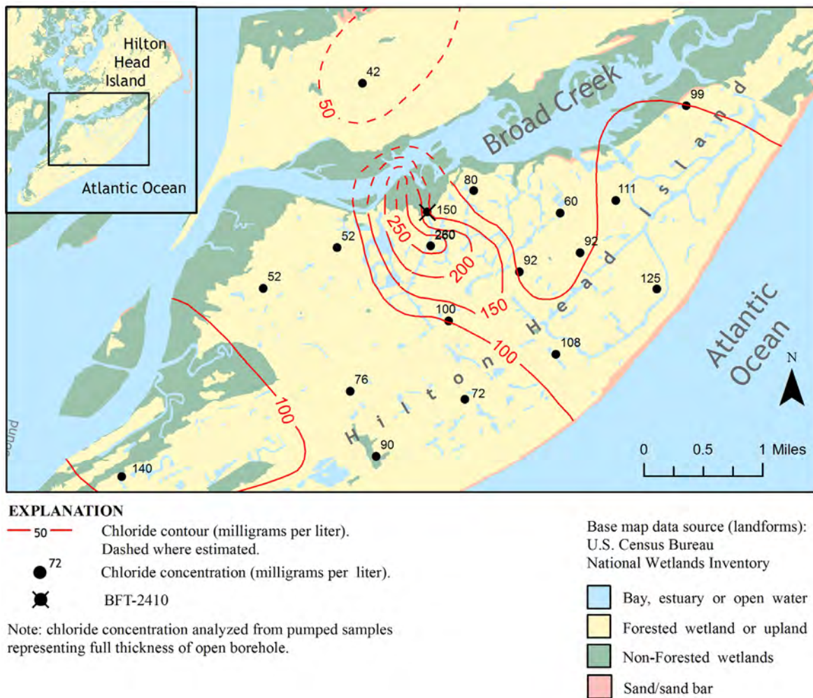
Figure 55. Location of test well BFT-2410 and isochlors showing the extent of the Broad Creek chloride plume, 2010, Hilton Head Island, S.C. (after Groundwater Management Associates, 2010).
