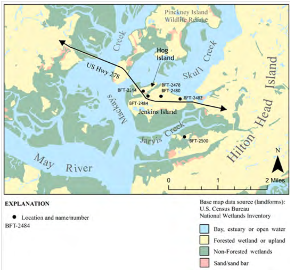
Figure 52. Locations of Upper Floridan aquifer and middle Floridan aquifer monitoring wells, Jenkins Island, S.C.
