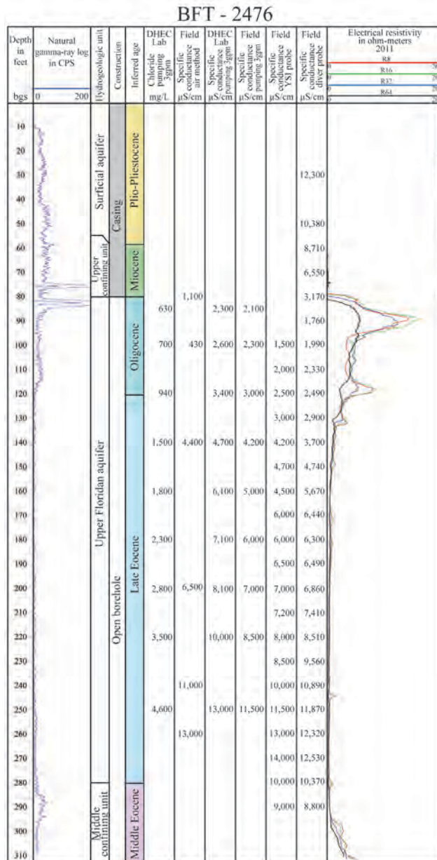
Figure 60. Hydrogeology, geophysical logs, specific conductance, chloride distribution, and well construction at well BFT-2476 near Bull Island, S.C. Bull Island, S.C.
