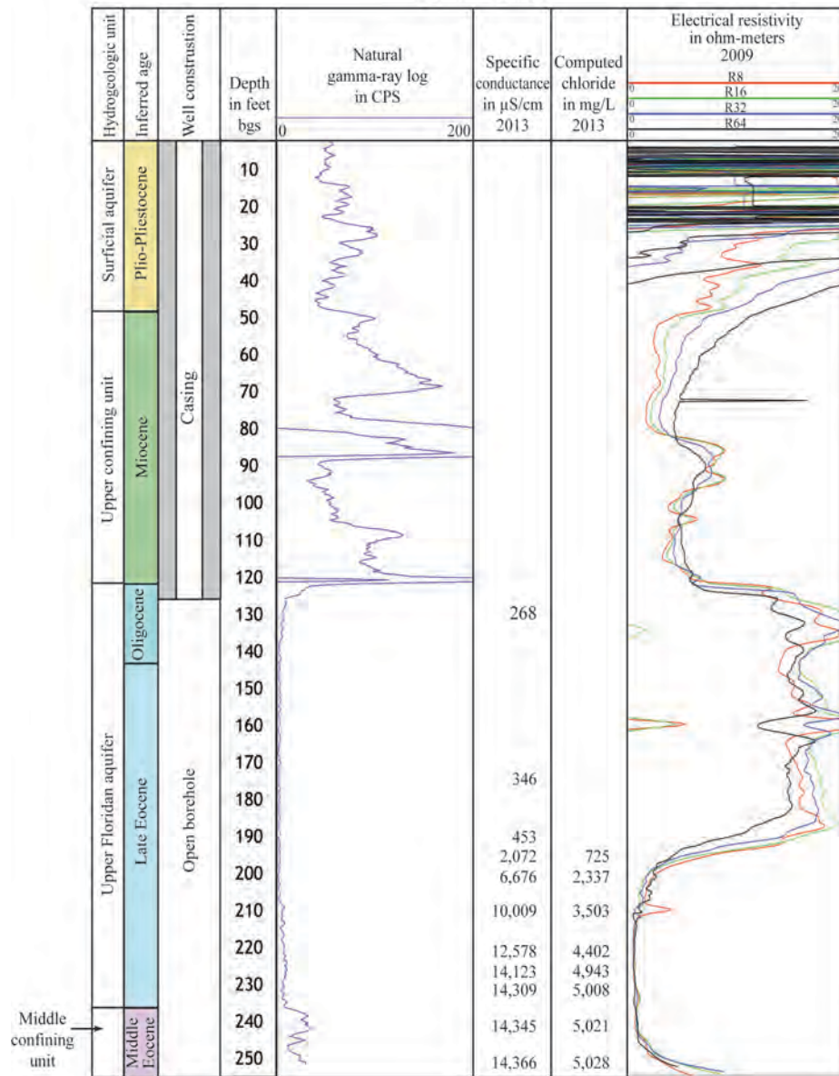
Figure 51. Hydrogeology, geophysical logs, chloride distribution, and well construction at well BFT-2408 near Sawmill Creek, S.C.
