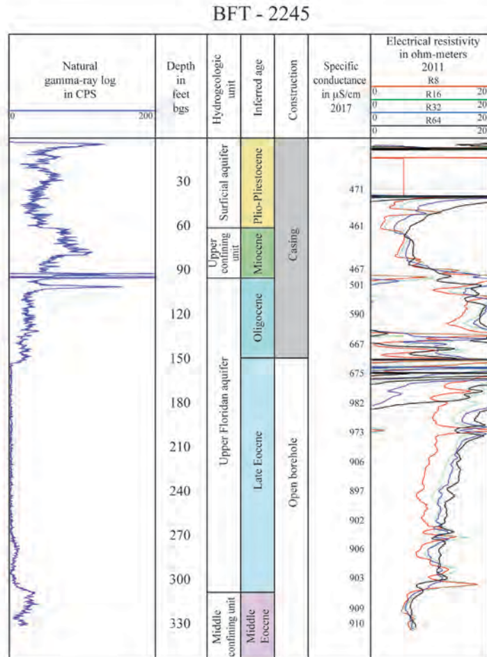
Figure 62. Geophysical logs and vertical specific-conductance profile at BFT-2245 on northern Daufuskie Island, S.C.
