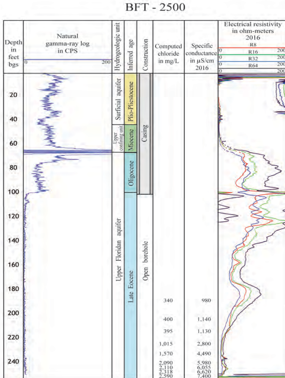
Figure 54. Hydrogeology, geophysical logs, chloride distribution, and well construction at well BFT-2500, near Jarvis Creek, Hilton Head Island, S.C.
