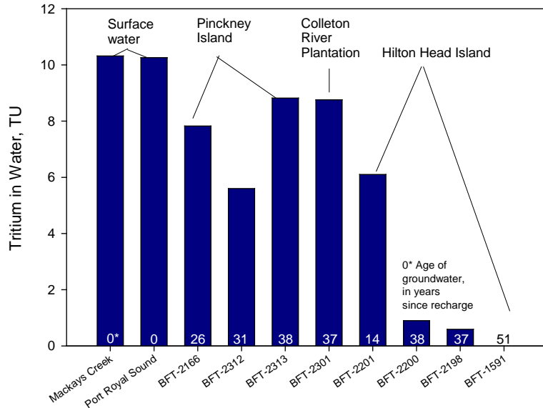
Figure 68. Recharge age computed from tritium concentrations in surface-water samples and Upper Floridan aquifer groundwater samples, southern Beaufort County, S.C., 2004–2005.
