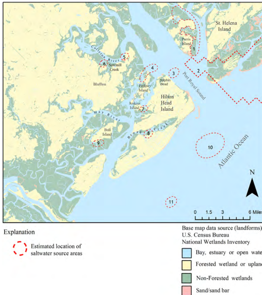
Figure 34. Estimated locations of saltwater source areas for the Upper Floridan aquifer, Port Royal Sound area, S.C.
