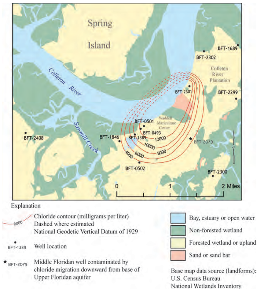
Figure 49. Isochors near the bottom of the Upper Floridan aquifer showing the extent of the Colleton River chloride plume, 2003, Colleton River Plantation, S.C.
