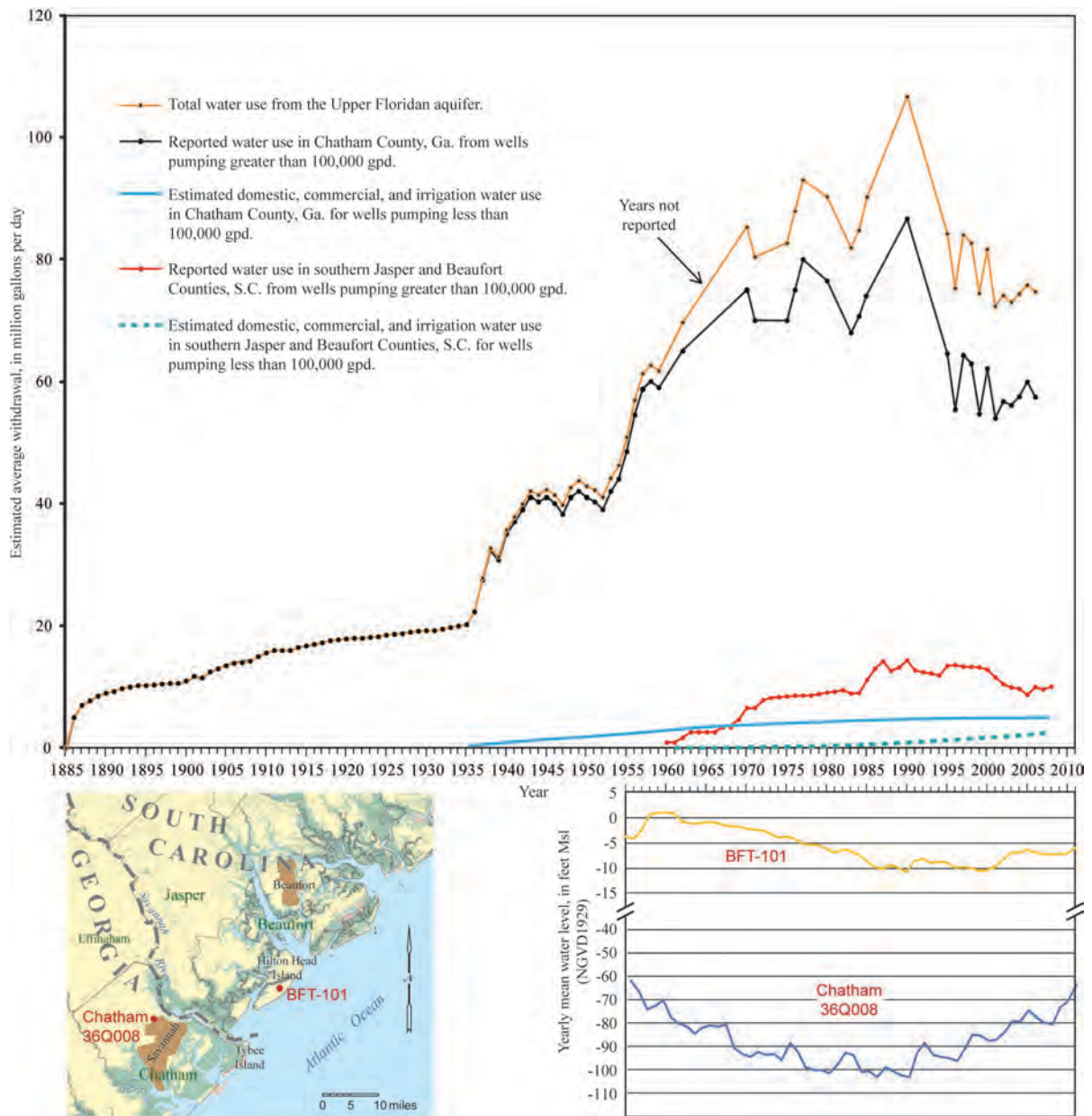
Figure 19. Upper Floridan aquifer water use in Chatham County, Ga., and southern Beaufort County, S.C., 1886–2006, and water levels in well BFT-101, Hilton Head Island, S.C., 1955-2007.
