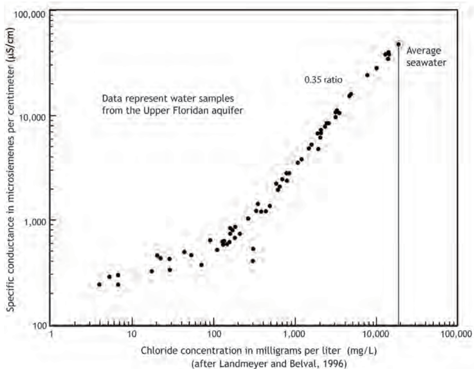
Figure 5. Chloride concentration vs. specific conductance in the Upper Floridan aquifer (Landmeyer and Belval, 1996).
