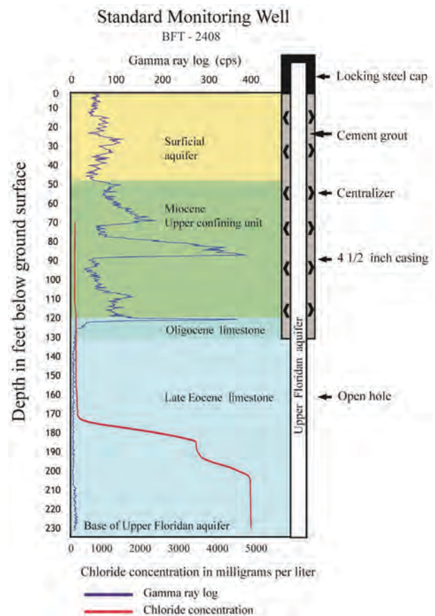
Figure 4. Well BFT-2408 showing standard monitoring-well construction, natural gamma-ray log, and chloride concentration computed from specific-conductance
