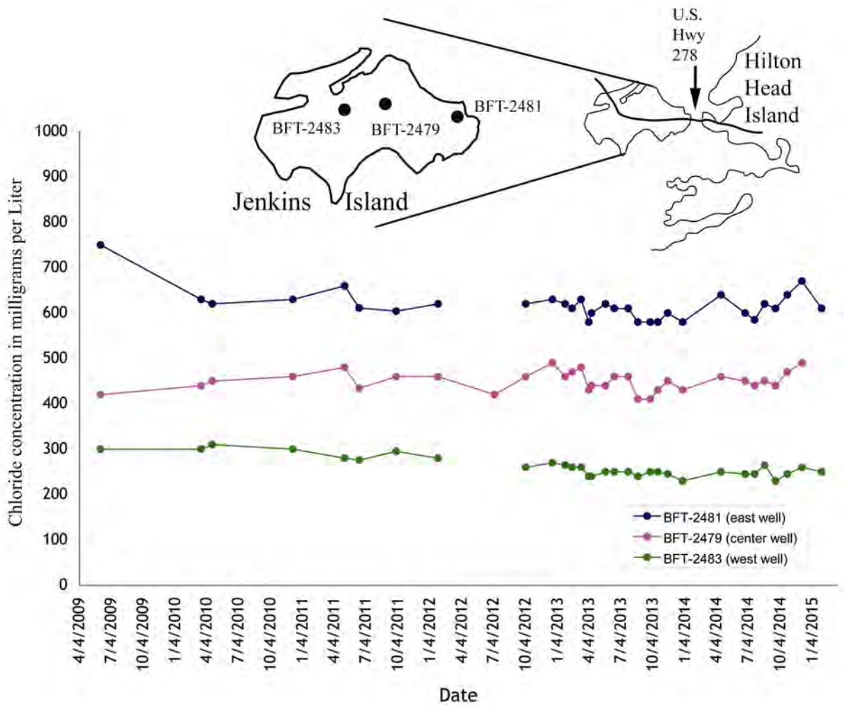
Figure 75. Chloride concentrations in middle Floridan aquifer wells at Jenkins Island, S.C., 2009–2015 (Hilton Head PSD data).
