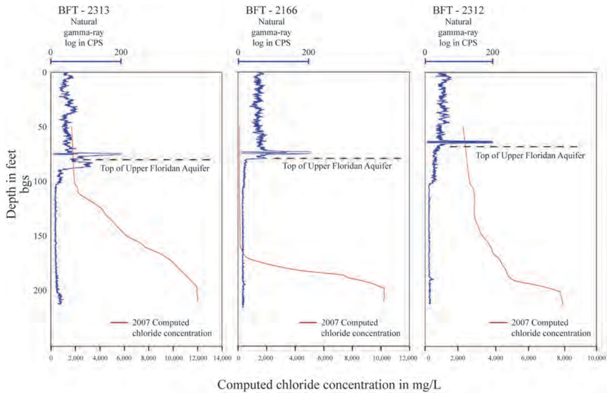
Figure 44. Chloride concentrations (red) and natural gamma-ray logs (blue) in Upper Floridan aquifer wells BFT-2313, BFT-2166, and BFT-2312, Pinckney Island, S.C., 2007. Concentrations computed from specific-conductance profiles.
