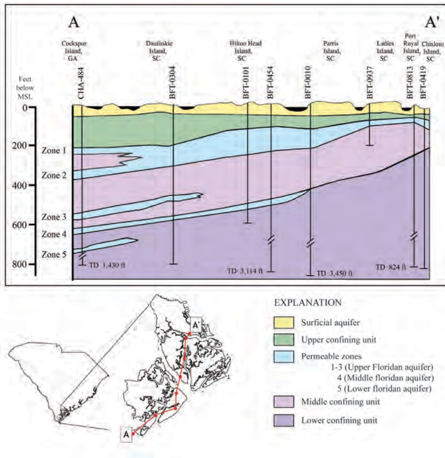
Figure 15. Permeable zones in the Floridan aquifer (after McCollum and Counts, 1964, pl. 4, and Hughes and others, 1989).
