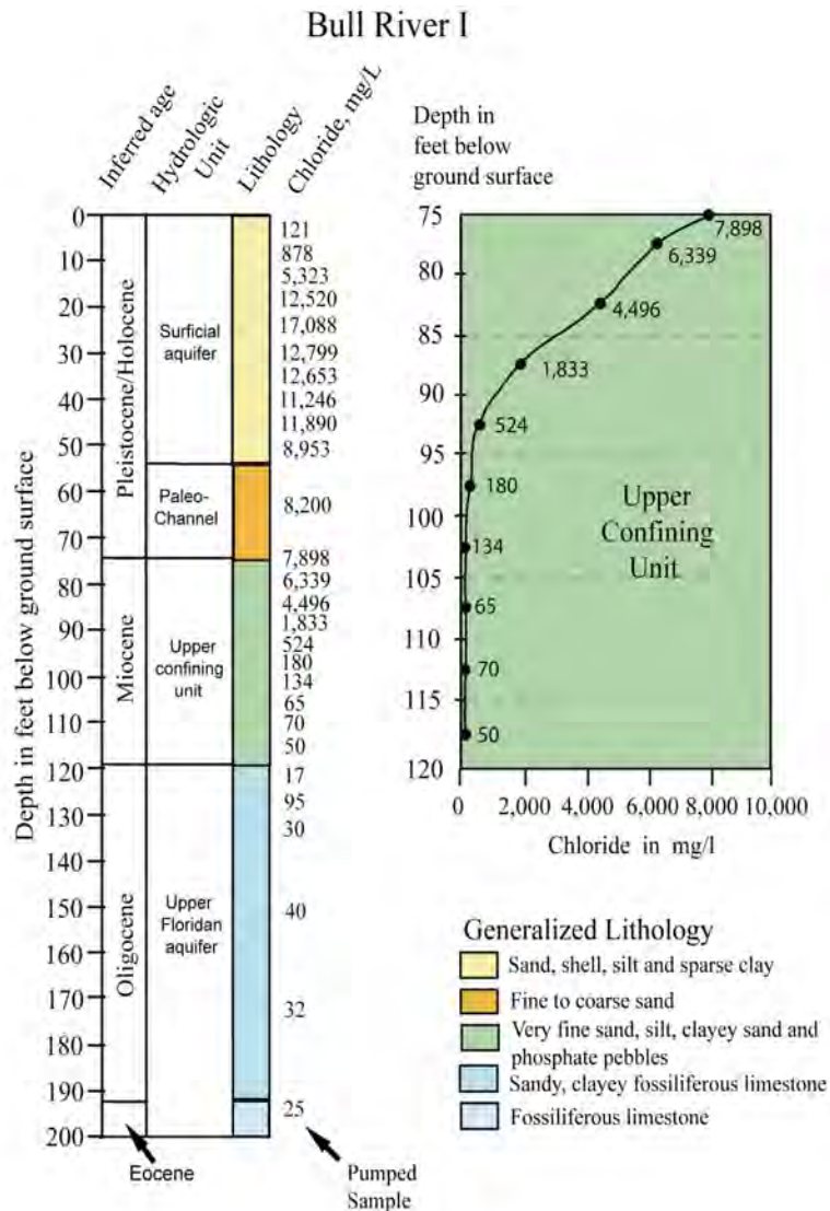
Figure 32. Chloride concentrations in pore-water samples from the surficial aquifer, upper confining unit, and Upper Floridan aquifer at well-site Bull River 1, 2005 (Ransom and others, 2006).
