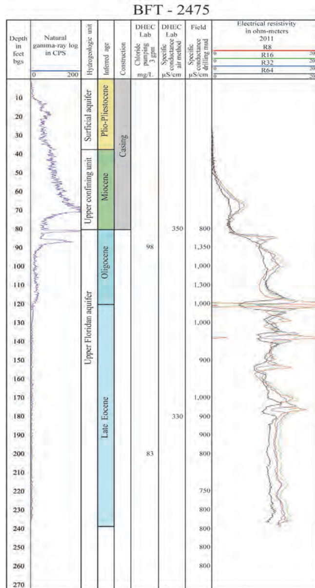
Figure 58. Hydrogeology, geophysical logs, specific conductance, chloride distribution, and well construction at well BFT-2475, Bull Island, S.C.
