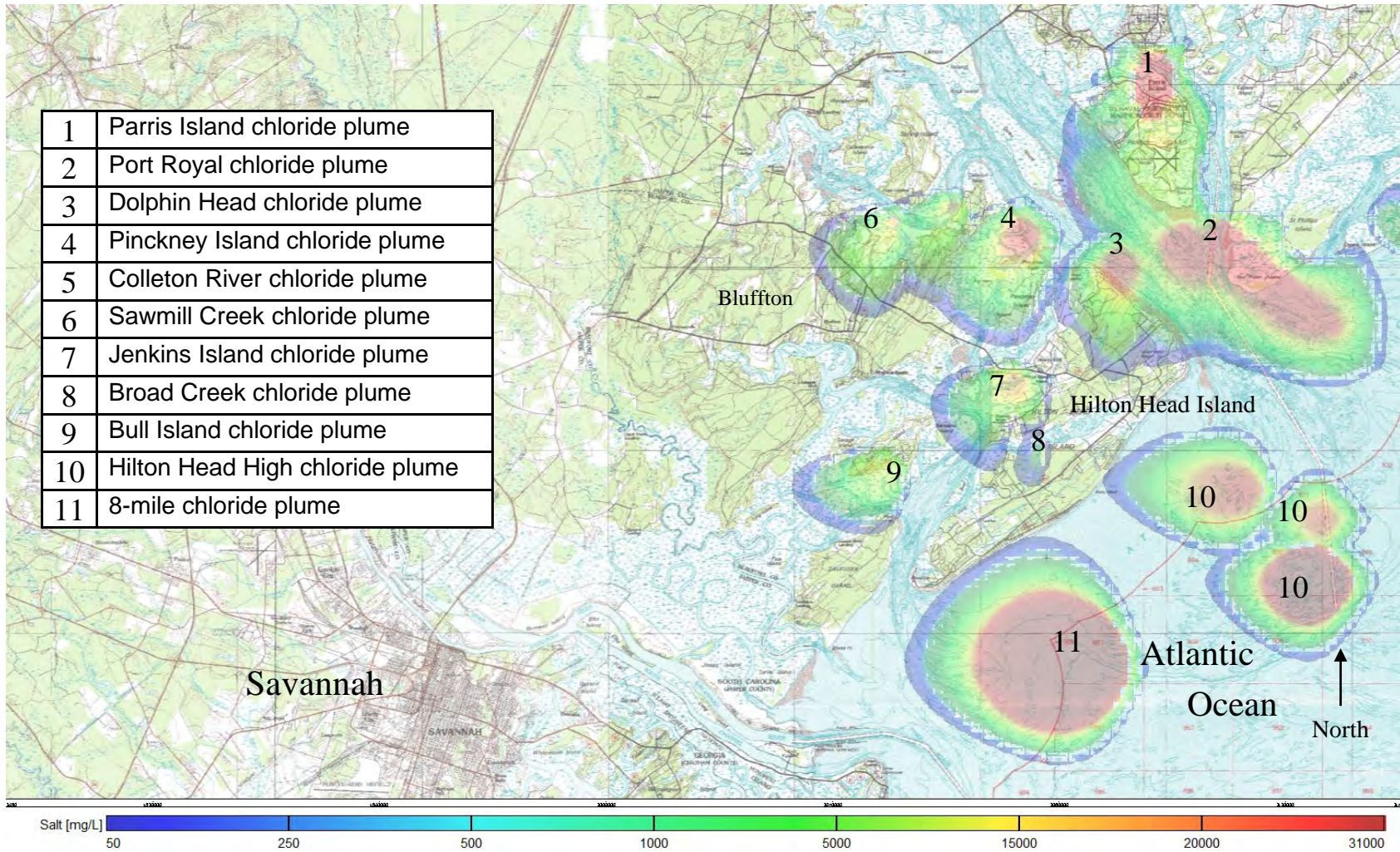
Figure J19. Simulated 2007 positions of brackish to saltwater plumes at the bottom of the Upper Floridan aquifer (permeable zone 2), Hilton Head Island S.C. – Savannah, Ga. area.
