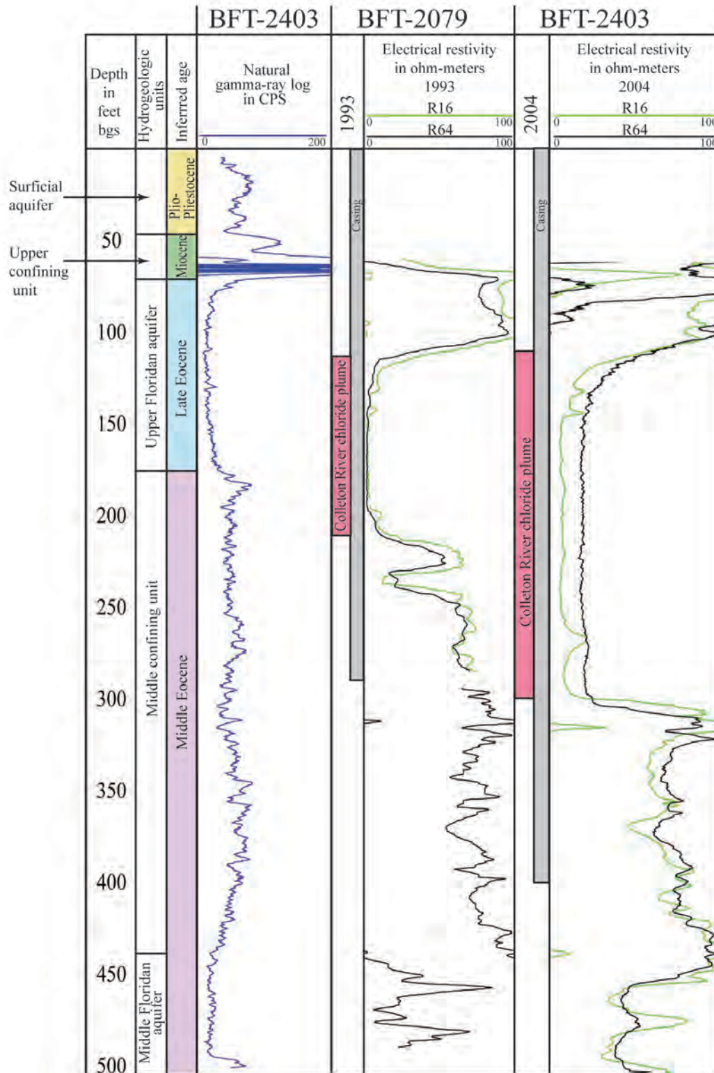
Figure 73. Changes in electrical resistivity (showing decreasing resistance) in the middle confining unit between 1993 and 2004 at Colleton River Plantation, S.C.
