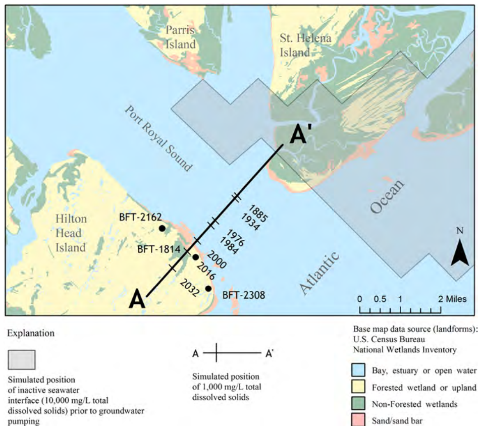
Figure 71. Simulated positions of the 1,000 mg/L total dissolved solids isopleth (saltwater-freshwater interface) beneath Port Royal Sound and Hilton Head Island, S.C. assuming 1984 pumpage, 1885–2032 (after Smith, 1988 and 1994).
