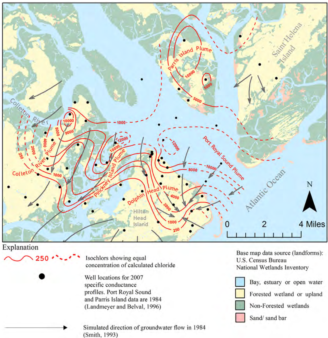
Figure 72. Isochlors map comprising the greater Port Royal Sound plume near the bottom of the Upper Floridan aquifer, Port Royal Sound area, S.C., 2007.
