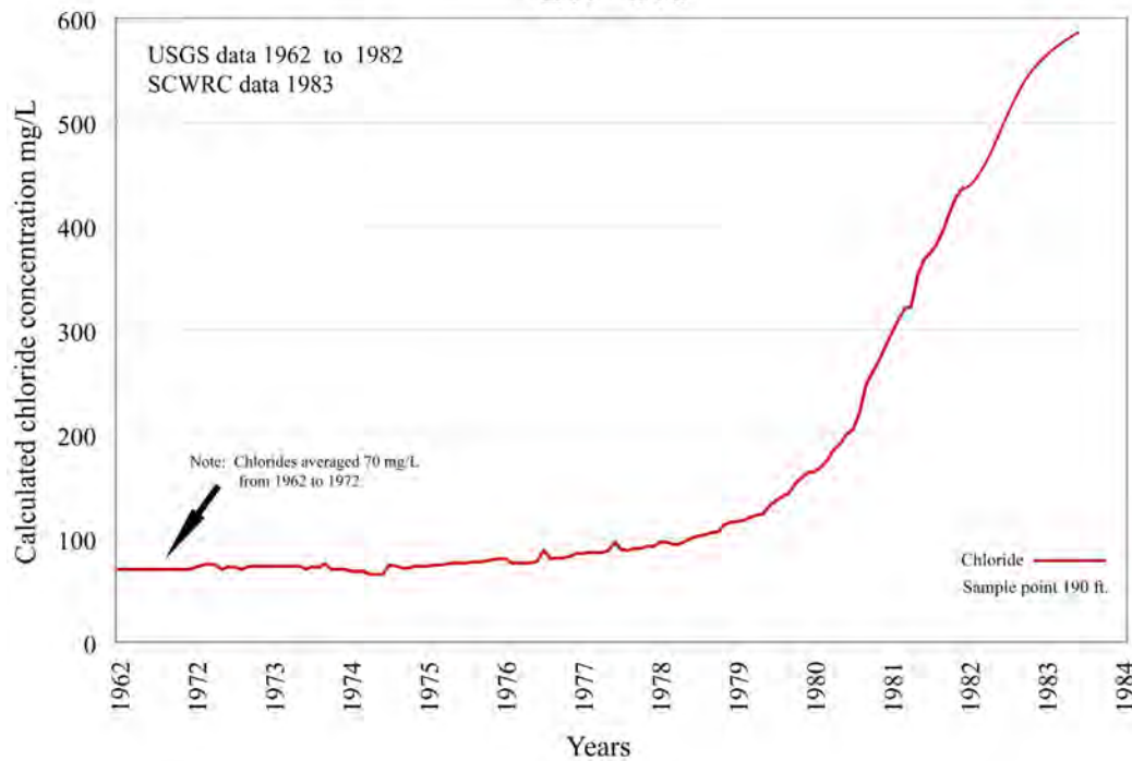
Figure 38. Chloride-concentration increases in the Upper Floridan aquifer at well BFT-315, 1962–1982, northern Hilton Head Island, S.C. (USGS data).
