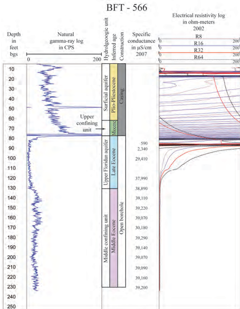
Figure 35. Natural gamma-ray log and vertical specific-conductance profile (2007) for monitor well BFT-566 at Parris Island, S.C.
