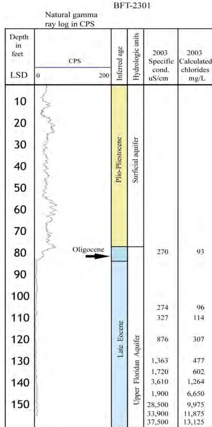
Figure 47. Hydrogeology, geophysical logs, specific conductance profile, and chloride distribution at well BFT-2301, near the Colleton River, S.C., 2003.
