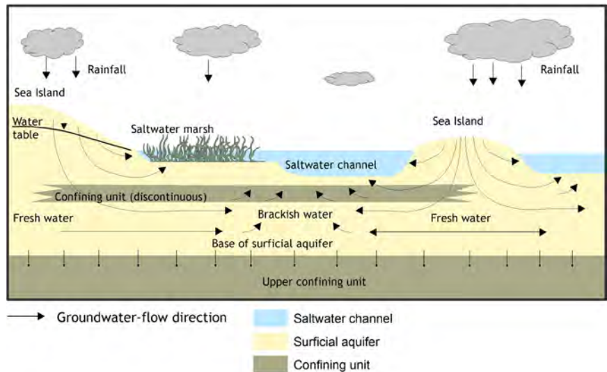
Figure 14. Schematic representation of groundwater flow in the surficial aquifer in response to recharge and discharge.
