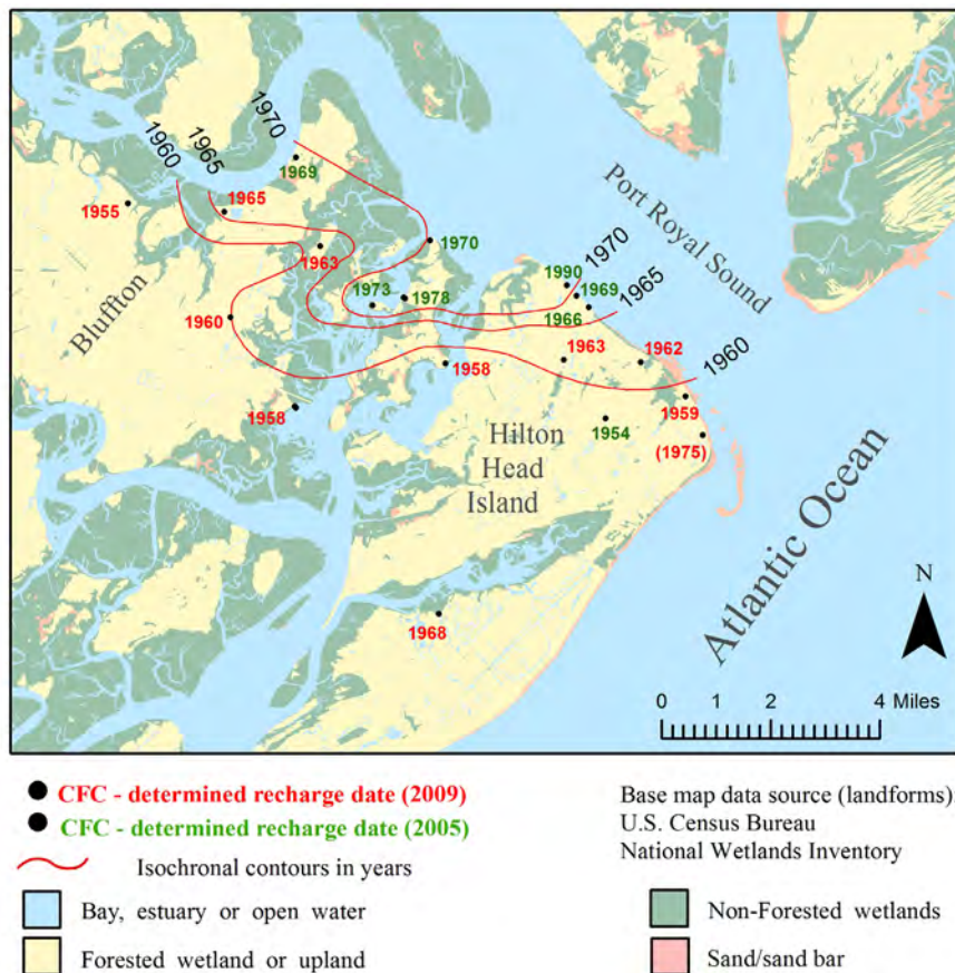
Figure 69. Isochronal contours representing equal saltwater recharge dates for water at the bottom of the Upper Floridan aquifer: determined by chlorofluorocarbon analyses (CFC-12), Port Royal Sound area, S.C.
