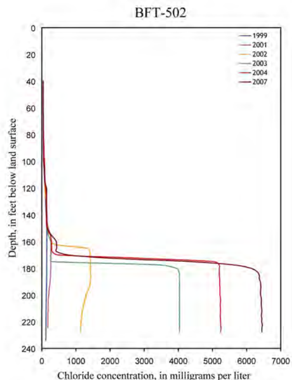
Figure 48. Computed chloride-concentration profiles in Upper Floridan aquifer well BFT-502, Colleton River area, S.C., 1999–2007.
