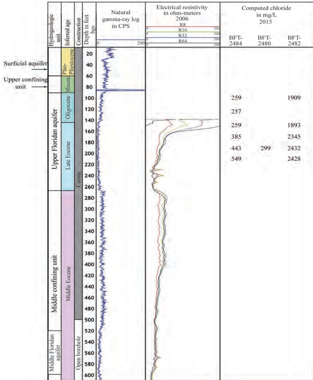
Figure 53. Hydrogeology, geophysical logs, chloride distribution, and well construction at well BFT-2478, Jenkins Island, S.C.
