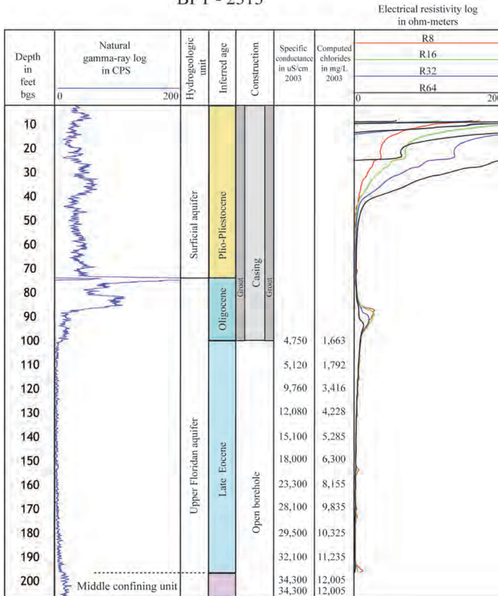
Figure 43. Hydrogeology, geophysical logs, chloride distribution, and well construction at well BFT-2313, Pinckney Island, S.C.
