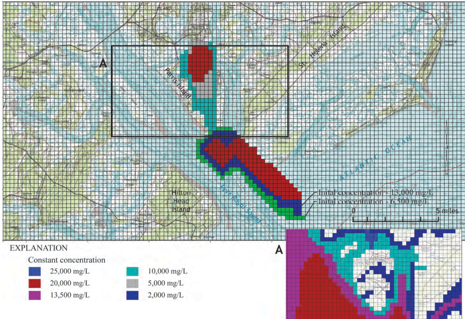
Figure J13. Initial and Constant concentrations assigned to the bottom of Upper Floridan aquifer and bottom of surficial aquifer for predevelopment conditions beneath Port Royal Sound and Paris Island, S.C.
