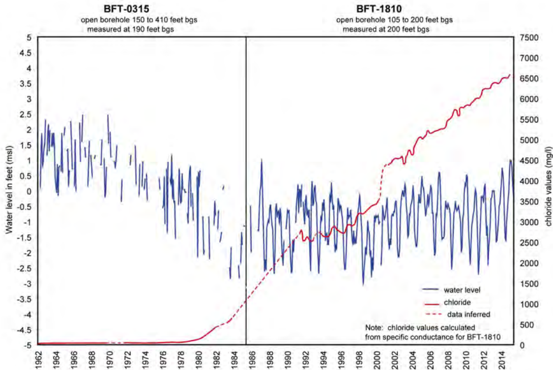
Figure 39. Water-level and computed chloride-concentration changes in BFT-315 and BFT-1810, 1962–2014, northern Hilton Head Island, S.C.
